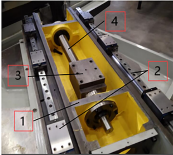
Fig 3. Linear guideways.
