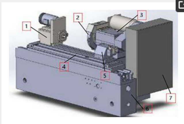
Fig 1. The overall three-dimensional model of grinding machine.
