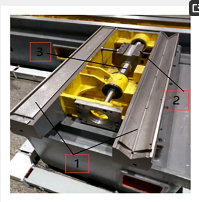
Fig 2. Integrated guideways.
