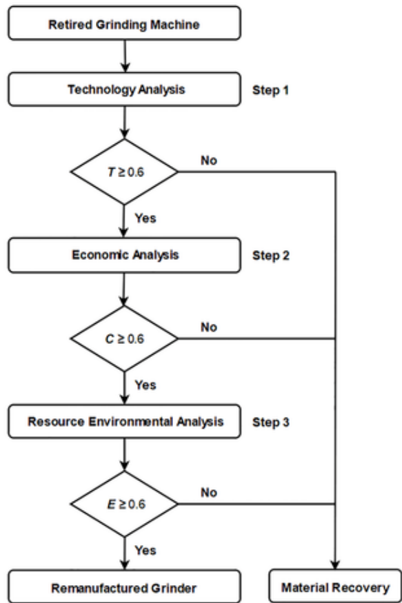
Fig 5. Evaluating process of grinding machine remanufacturability. https://doi.org/10.1371/journal.pone.0234603.g005
